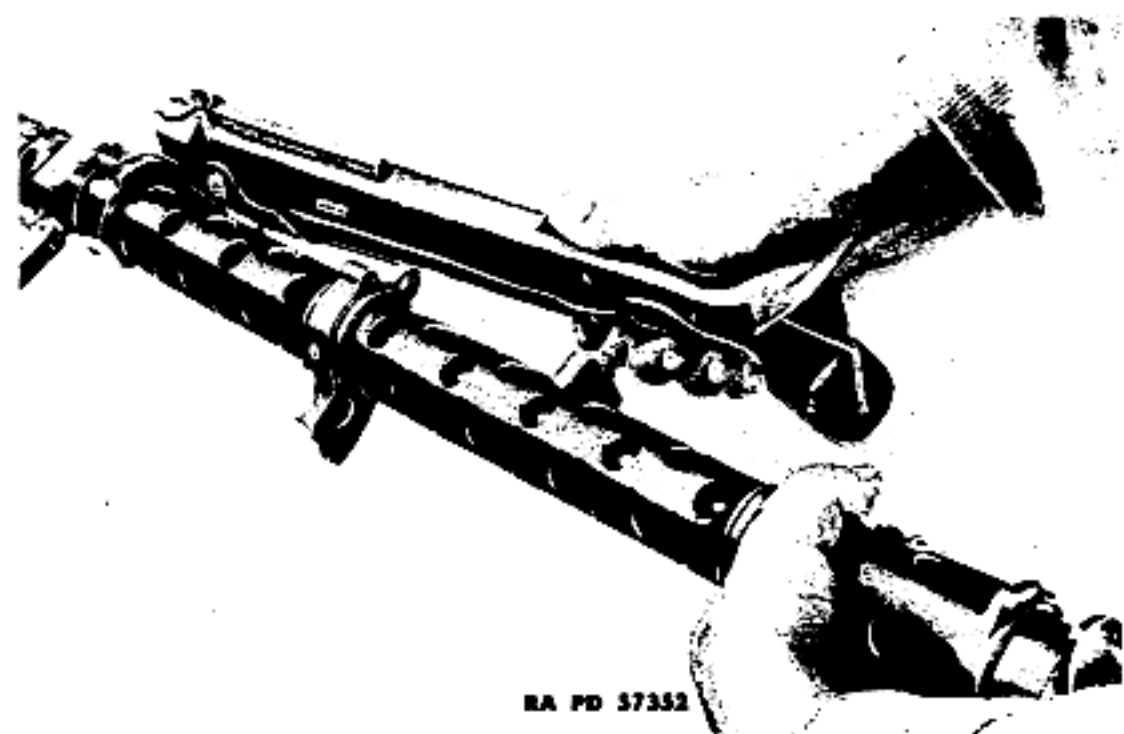
Figure 7 - Attaching Bipod Legs to Barrel Casing
